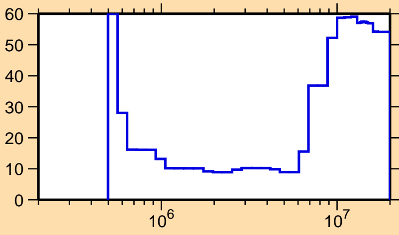
\Delta\sigma/\sigma vs. E for ^{110}\text{Ag}(n,n\text{cont.})
