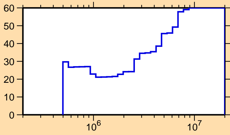
\Delta\sigma/\sigma vs. E for ^{110}\text{Ag}(n,n_1)
