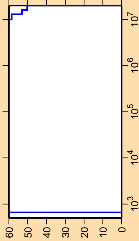
\Delta\sigma/\sigma vs. E for ^{110}\text{Ag}(n,\alpha)
