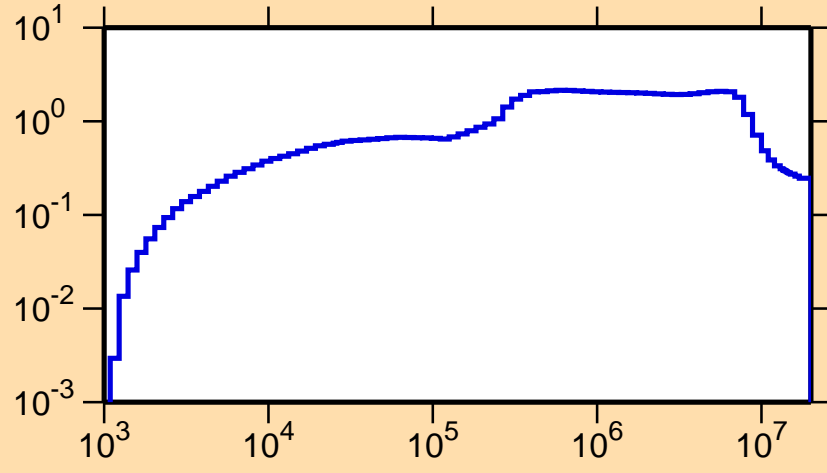
\sigma vs. E for ^{110}\text{Ag}(n,\text{inel.})
