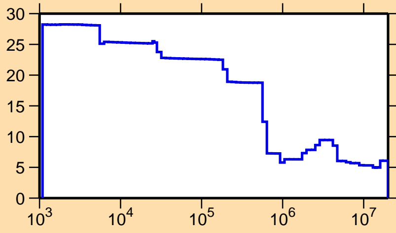
\Delta\sigma/\sigma vs. E for ^{110}\text{Ag}(n,\text{nonel.})
