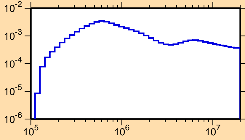
\sigma vs. E for ^{110}\text{Ag}(n,n_2)
