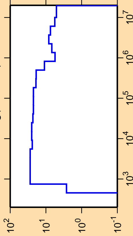
\Delta\sigma/\sigma vs. E for ^{110}\text{Ag}(n,\text{nonel.})
