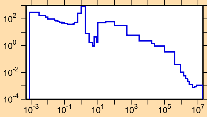
\sigma vs. E for ^{110}\text{Ag}(n,\gamma)
