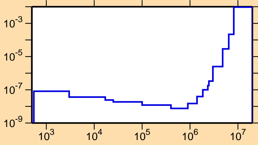
\sigma vs. E for ^{110}\text{Ag}(n,\alpha)
