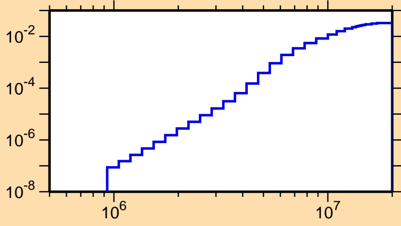
\sigma vs. E for ^{110}\text{Ag}(n,p)
