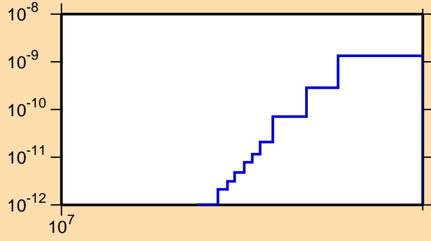
\sigma vs. E for ^{110}\text{Ag}(n,p\alpha)
