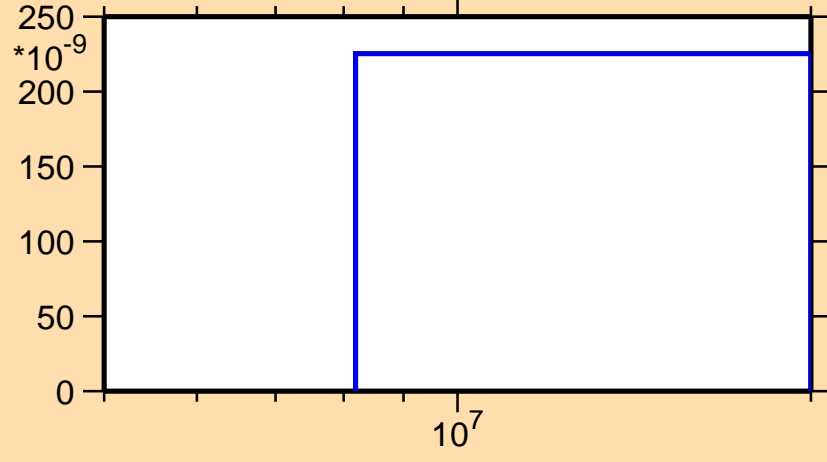
\sigma vs. E for ^{110}\text{Ag}(n,2np)
