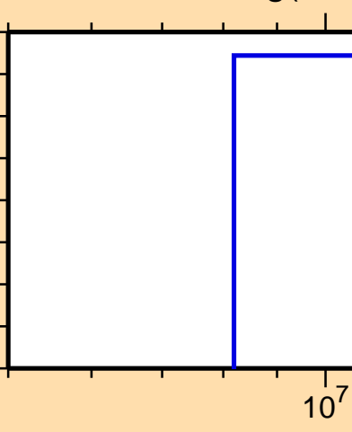
\sigma vs. E for ^{110}\text{Ag}(n,np)
