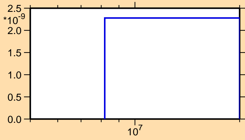
\sigma vs. E for ^{110}\text{Ag}(n,nt)
