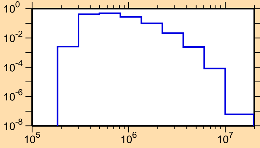
\sigma vs. E for ^{111}\text{Ag}(n,n_3)
