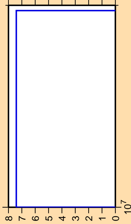
\Delta\sigma/\sigma vs. E for ^{111}\text{Ag}(n,2n\alpha)
