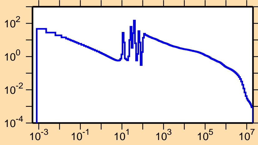
\sigma vs. E for ^{111}\text{Ag}(n,\gamma)
