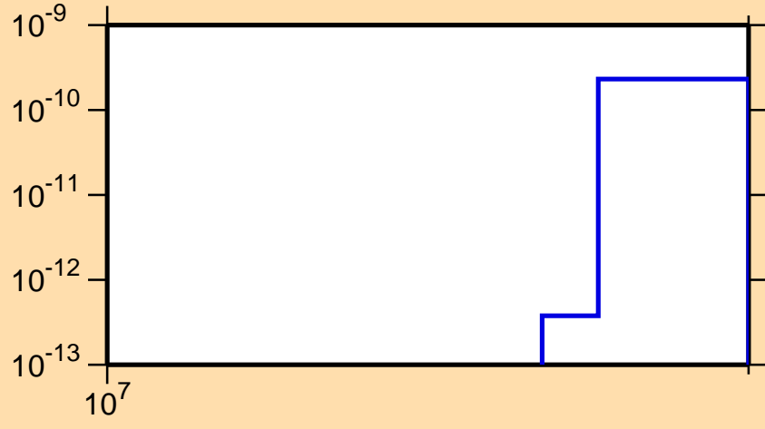
\sigma vs. E for ^{112}\text{Ag}(n,\text{He}3)
