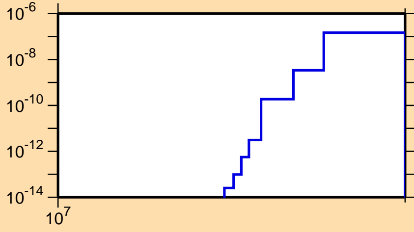
\sigma vs. E for ^{112}\text{Ag}(n,2n\alpha)
