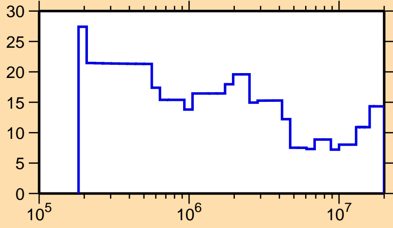
\Delta\sigma/\sigma vs. E for ^{112}\text{Ag}(n,el.)
