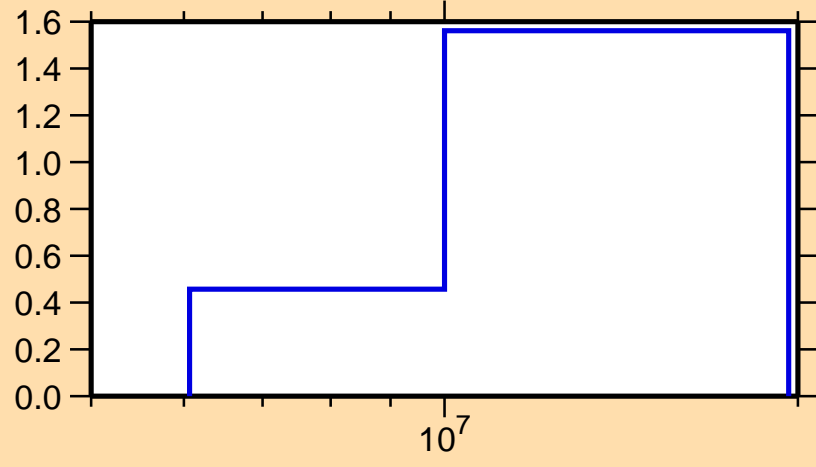
\sigma vs. E for ^{112}\text{Ag}(n,2n)
