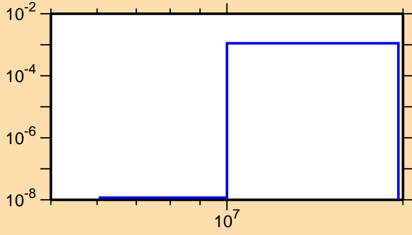
\sigma vs. E for ^{112}\text{Ag}(n,d)
