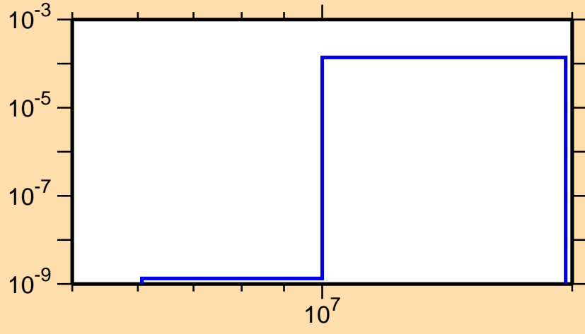
\sigma vs. E for ^{112}\text{Ag}(n,t)
