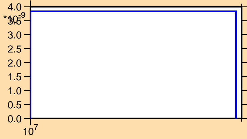
\sigma vs. E for ^{112}\text{Ag}(n,nt)
