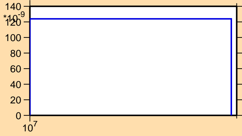
\sigma vs. E for ^{112}\text{Ag}(n,2np)
