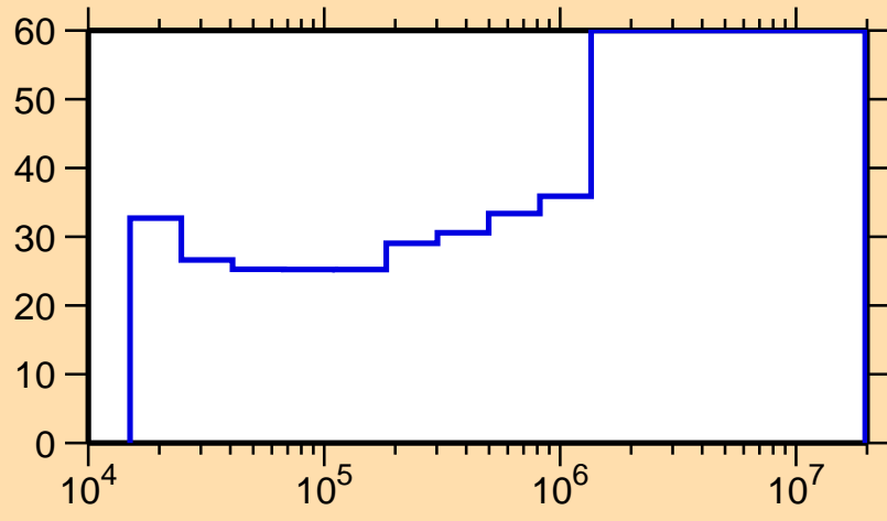
\Delta\sigma/\sigma vs. E for ^{112}\text{Ag}(n,n_1)
