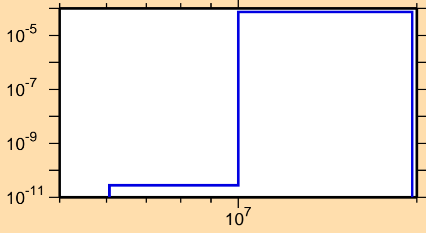
\sigma vs. E for ^{112}\text{Ag}(n,n\alpha)
