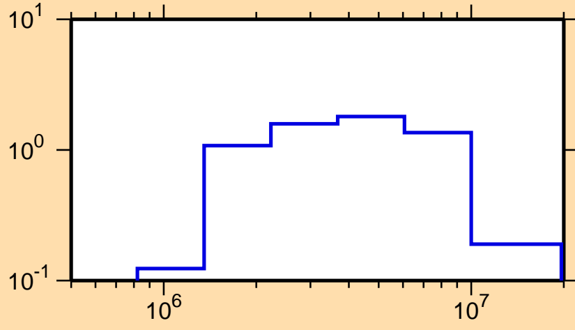
\sigma vs. E for ^{112}\text{Ag}(n,n\text{cont.})
