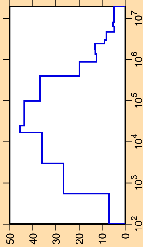
\Delta\sigma/\sigma vs. E for ^{112}\text{Ag}(n,\text{nonel.})
