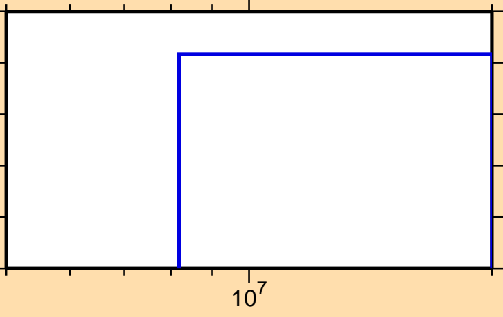
\sigma vs. E for ^{112}\text{Ag}(n,nt)
