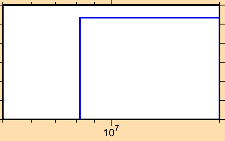
\sigma vs. E for ^{112}\text{Ag}(n,3n)
