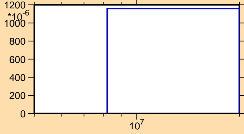
\sigma vs. E for ^{112}\text{Ag}(n,np)
