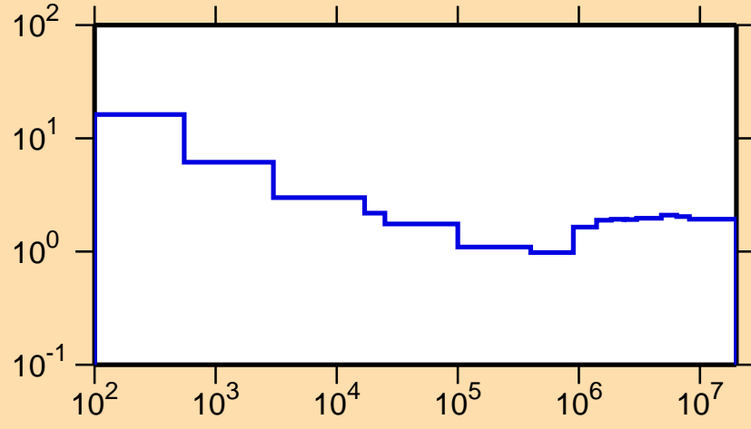
\sigma vs. E for ^{112}\text{Ag}(n,\text{nonel.})
