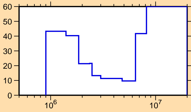
\Delta\sigma/\sigma vs. E for ^{112}\text{Ag}(n,n\text{cont.})
