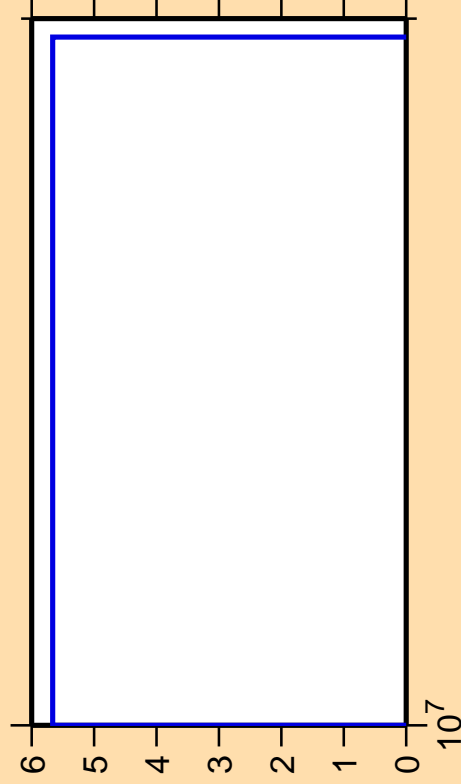
\Delta\sigma/\sigma vs. E for ^{113}\text{Ag}(n,2n\alpha)
