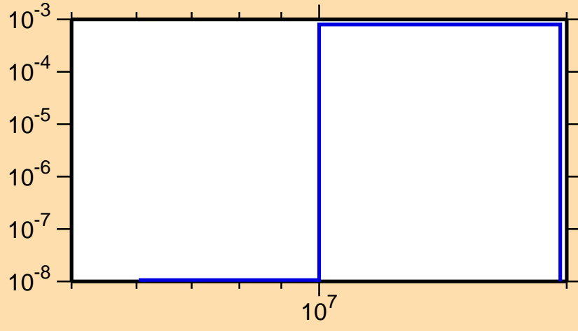
\sigma vs. E for ^{113}\text{Ag}(n,d)
