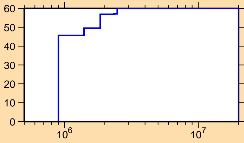
\Delta\sigma/\sigma vs. E for ^{113}\text{Ag}(n,n_1)
