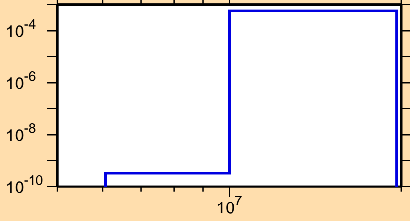
\sigma vs. E for ^{113}\text{Ag}(n,d)
