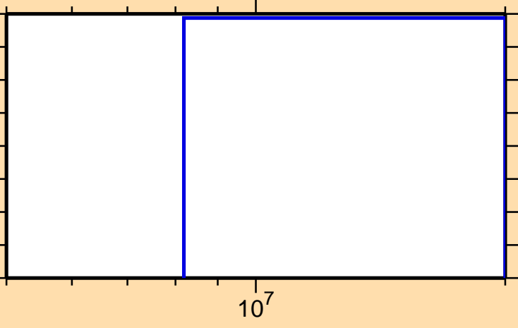
\sigma vs. E for ^{113}\text{Ag}(n,3n)
