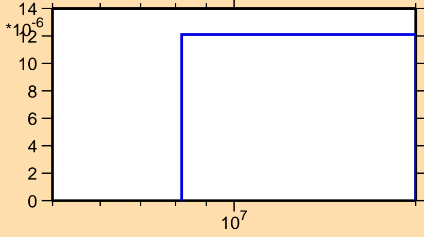
\sigma vs. E for ^{113}\text{Ag}(n,t)
