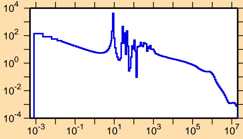
\sigma vs. E for ^{114}\text{Ag}(n,\gamma)
