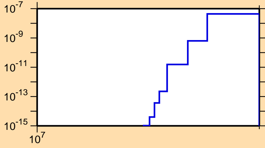
\sigma vs. E for ^{114}\text{Ag}(n,2n\alpha)
