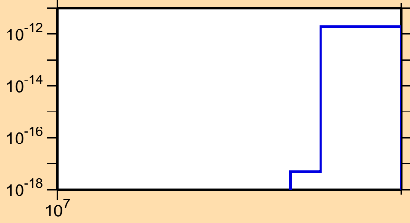
\sigma vs. E for ^{114}\text{Ag}(n,\text{He}3)
