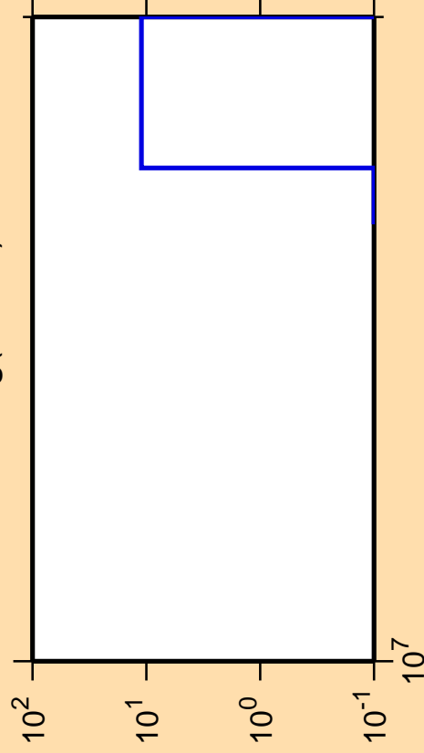
\Delta\sigma/\sigma vs. E for ^{114}\text{Ag}(n,\text{He}3)
