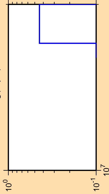
\Delta\sigma/\sigma vs. E for ^{114}\text{Ag}(n,p\alpha)
