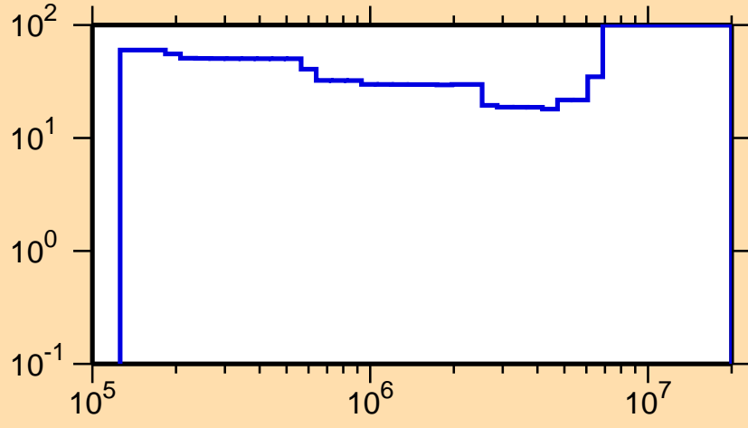
\Delta\sigma/\sigma vs. E for ^{114}\text{Ag}(n,\text{inel.})
