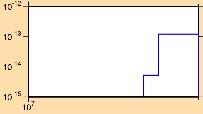
\sigma vs. E for ^{114}\text{Ag}(n,p\alpha)
