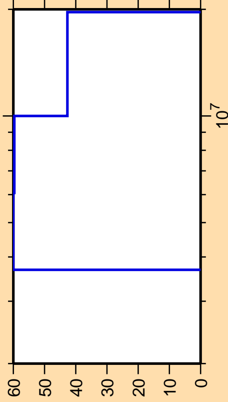
\Delta\sigma/\sigma vs. E for ^{114}\text{Ag}(n,2n)
