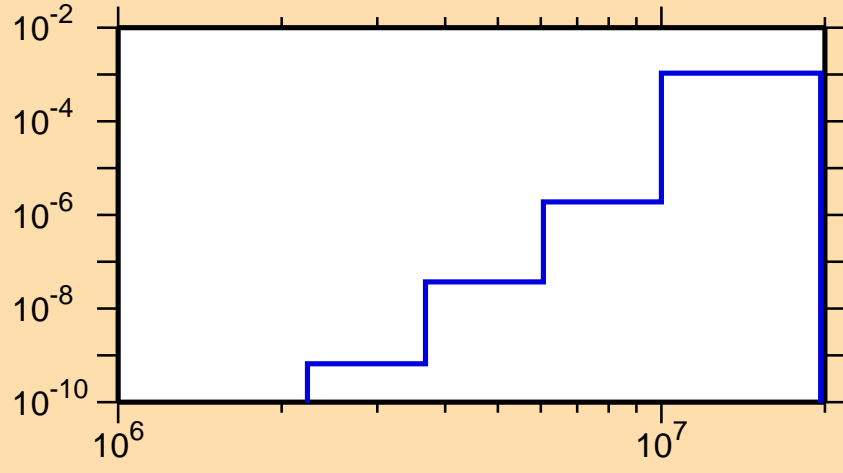
\sigma vs. E for ^{114}\text{Ag}(n,\alpha)
