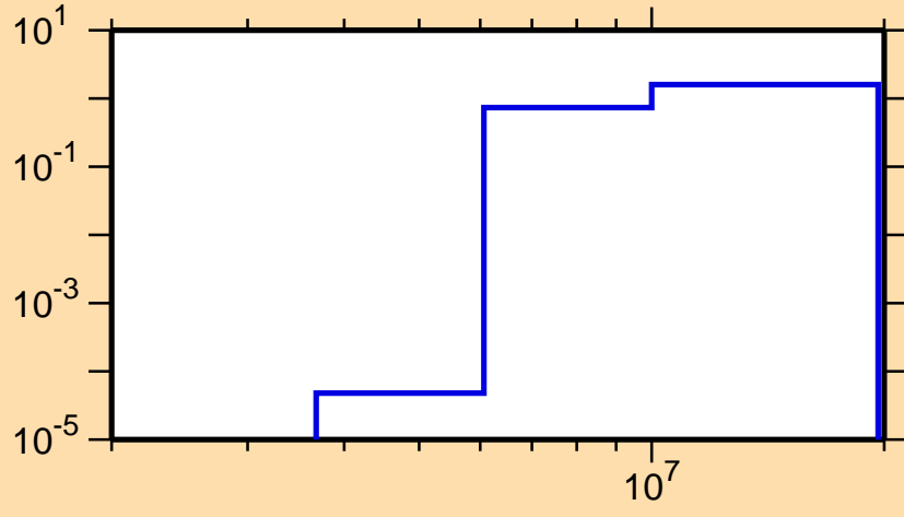
\sigma vs. E for ^{114}\text{Ag}(n,2n)
