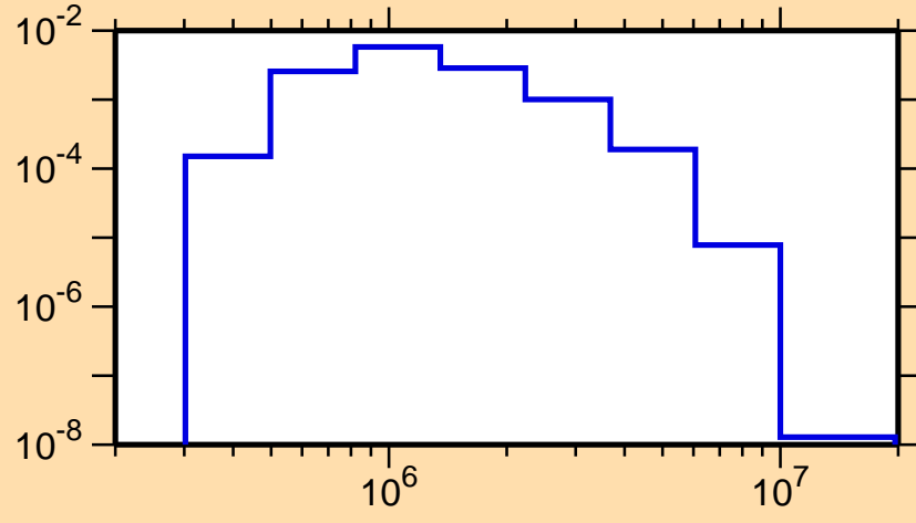
\sigma vs. E for ^{114}\text{Ag}(n,n_4)
