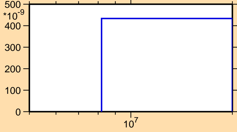
\sigma vs. E for ^{114}\text{Ag}(n,\text{nd})
