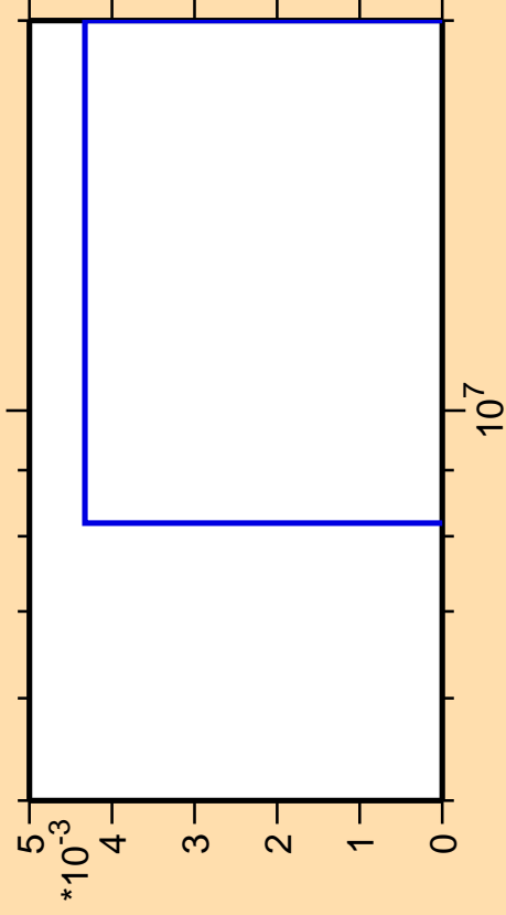
\Delta\sigma/\sigma vs. E for ^{114}\text{Ag}(n,p\alpha)
