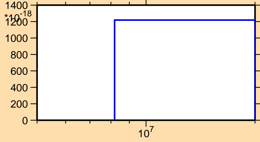
\sigma vs. E for ^{114}\text{Ag}(n,p\alpha)
