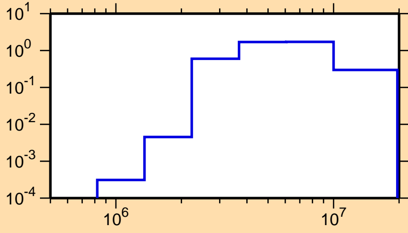
\sigma vs. E for ^{115}\text{Ag}(n,n\text{cont.})
