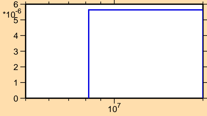
\sigma vs. E for ^{115}\text{Ag}(n,t)
