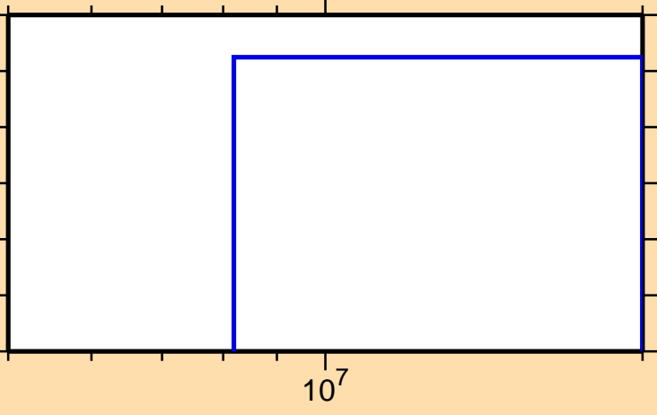
\sigma vs. E for ^{115}\text{Ag}(n,n\alpha)
