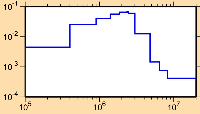
\sigma vs. E for ^{115}\text{Ag}(n,n_2)
