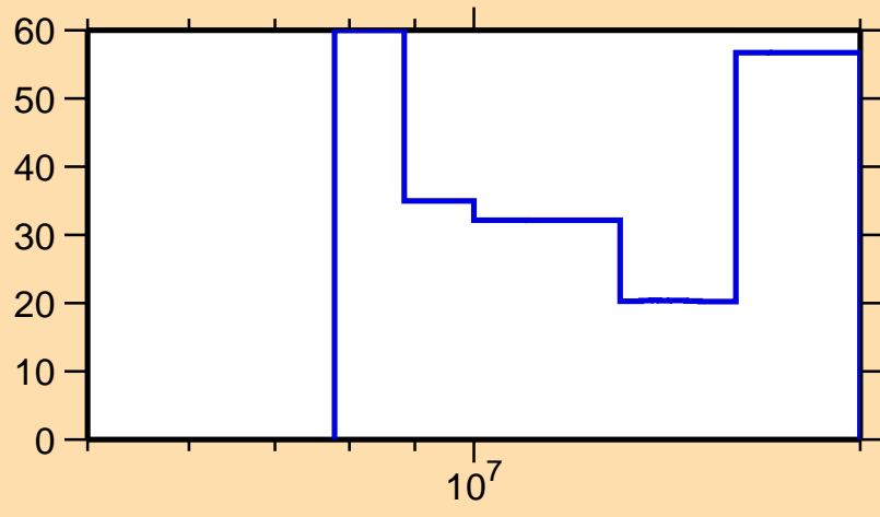
\Delta\sigma/\sigma vs. E for ^{115}\text{Ag}(n,2n)
