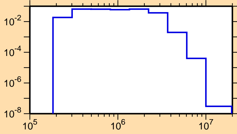
\sigma vs. E for ^{115}\text{Ag}(n,n_3)
