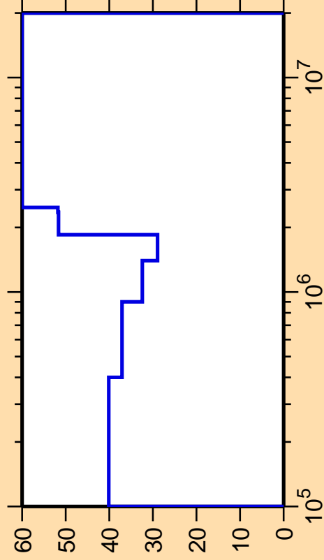
\Delta\sigma/\sigma vs. E for ^{115}\text{Ag}(n,n_4)
