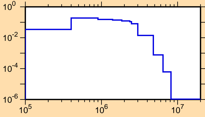
\sigma vs. E for ^{115}\text{Ag}(n,n_4)
