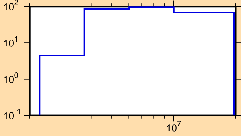
\Delta\sigma/\sigma vs. E for ^{116}\text{Ag}(n,p)
