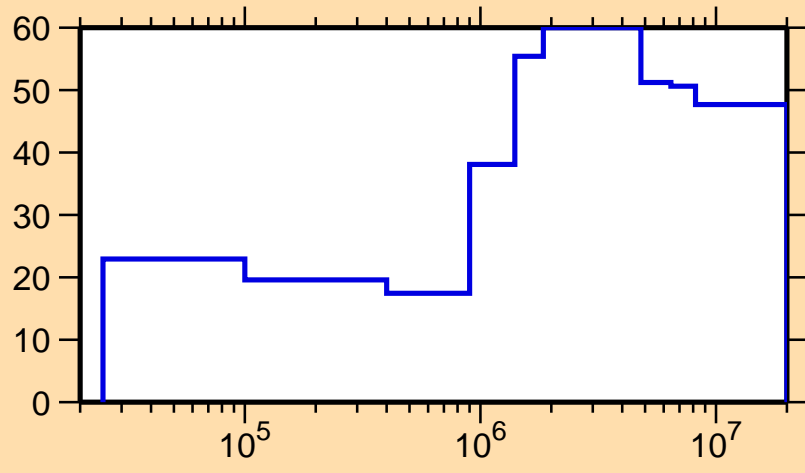
\Delta\sigma/\sigma vs. E for ^{116}\text{Ag}(n,n_1)
