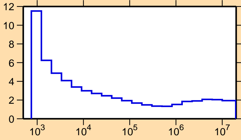
\sigma vs. E for ^{116}\text{Ag}(n,\text{nonel.})
