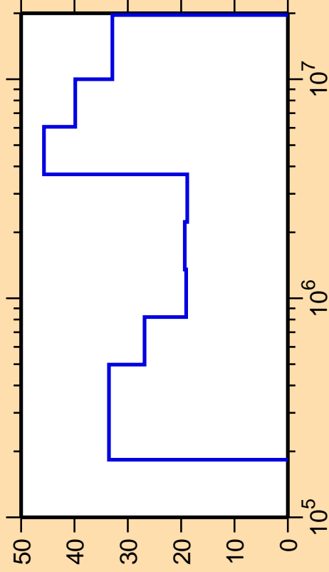
\Delta\sigma/\sigma vs. E for ^{117}\text{Ag}(n,n_2)
