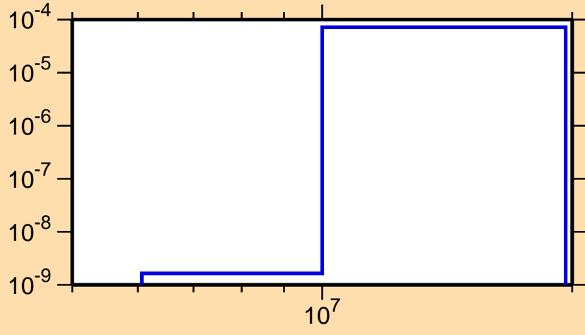
\sigma vs. E for ^{117}\text{Ag}(n,\alpha)
