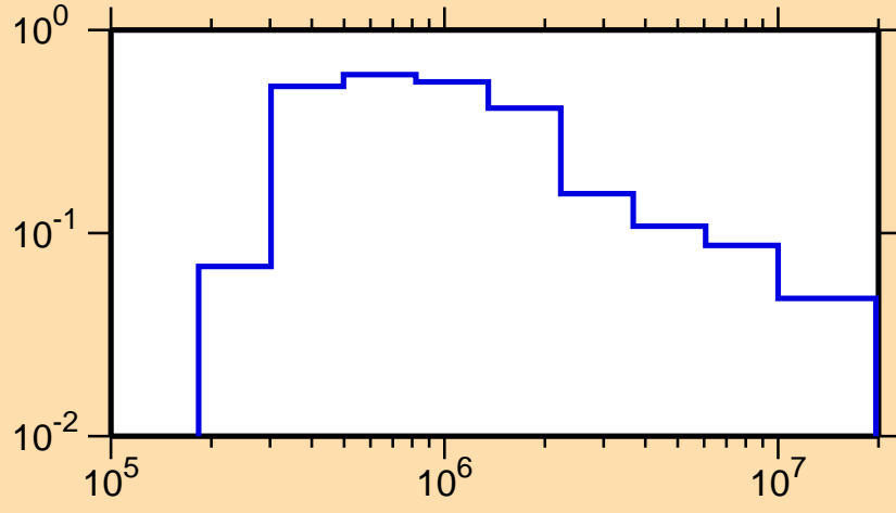
\sigma vs. E for ^{117}\text{Ag}(n,n_2)
