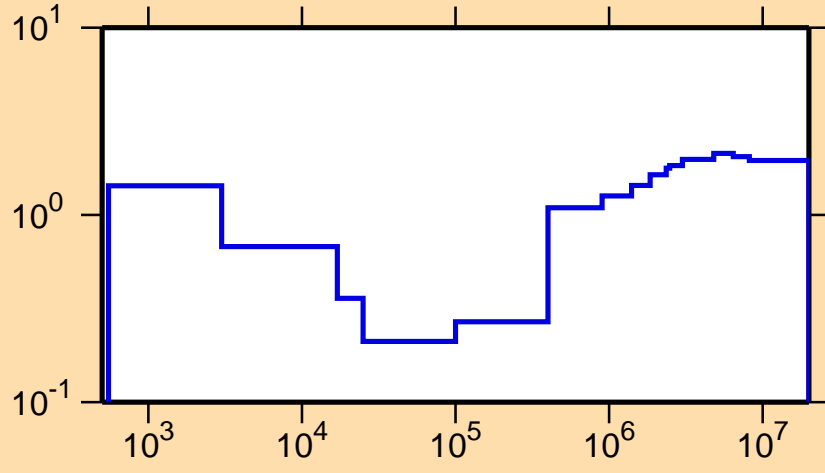
\sigma vs. E for ^{117}\text{Ag}(n,\text{nonel.})
