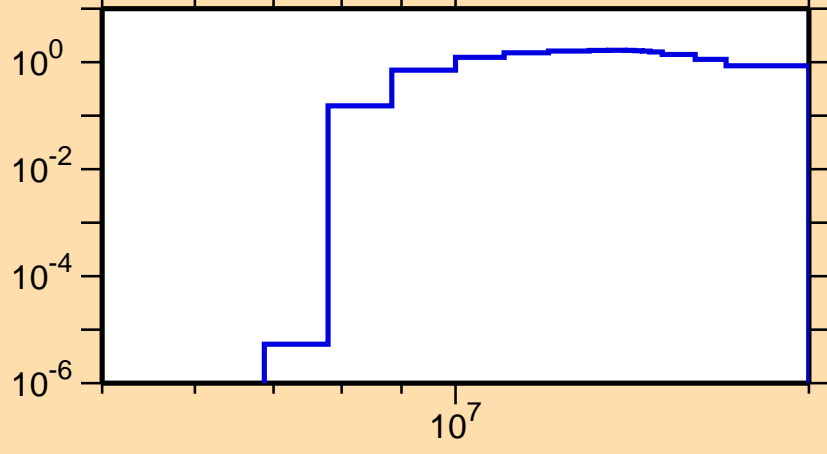
\sigma vs. E for ^{117}\text{Ag}(n,2n)
