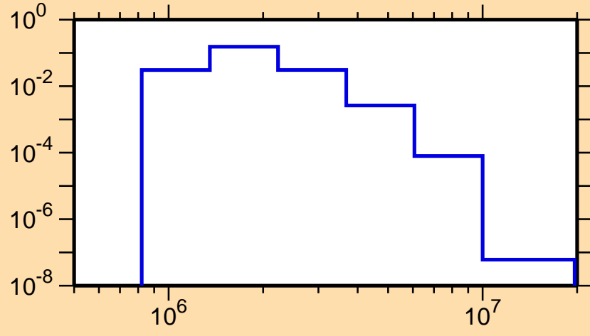
\sigma vs. E for ^{117}\text{Ag}(n,n_4)
