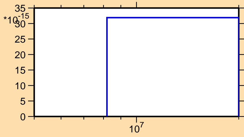
\sigma vs. E for ^{117}\text{Ag}(n,2n\alpha)
