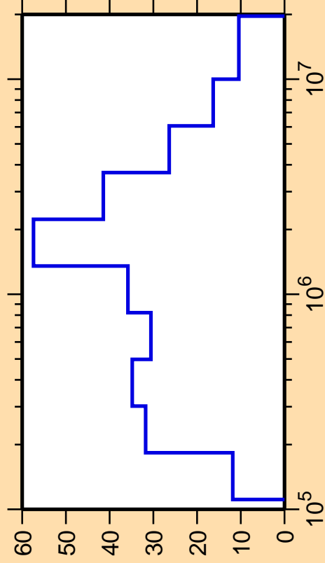
\Delta\sigma/\sigma vs. E for ^{118}\text{Ag}(n,n_4)
