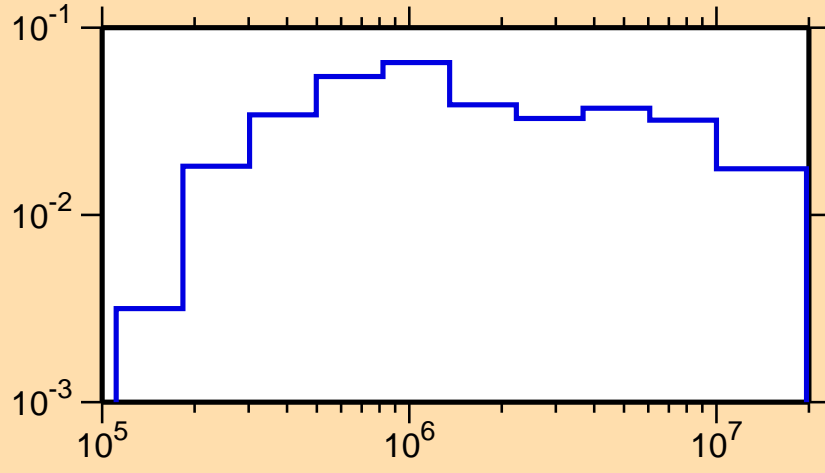
\sigma vs. E for ^{118}\text{Ag}(n,n_4)
