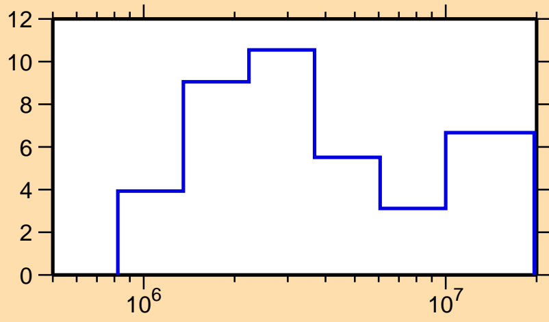
\Delta\sigma/\sigma vs. E for ^{118}\text{Ag}(n, tot.)
