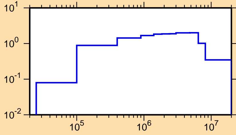
\sigma vs. E for ^{118}\text{Ag}(n,\text{inel.})
