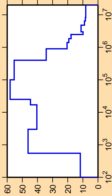
\Delta\sigma/\sigma vs. E for ^{118}\text{Ag}(n,\text{nonel.})
