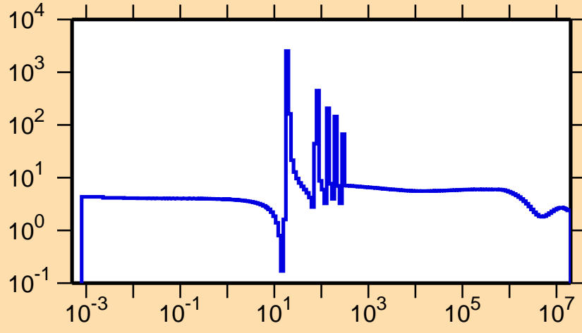
\sigma vs. E for ^{118}\text{Ag}(n,\text{el.})
