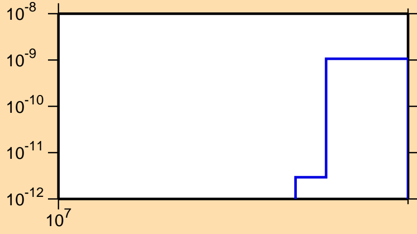
\sigma vs. E for ^{118}\text{Ag}(n,2n\alpha)
