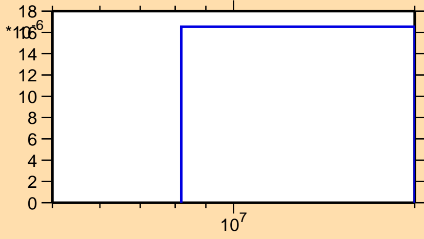
\sigma vs. E for ^{118}\text{Ag}(n,t)
