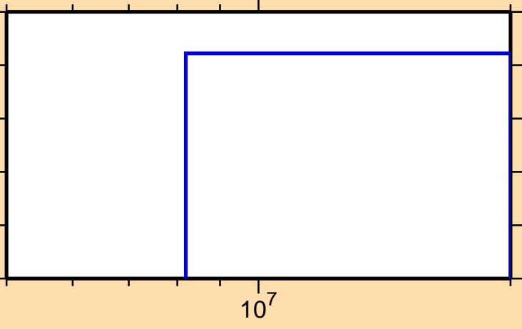
\sigma vs. E for ^{118}\text{Ag}(n,np)
