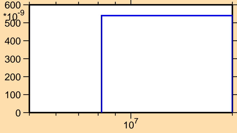
\sigma vs. E for ^{118}\text{Ag}(n,n\alpha)
