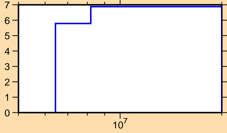
\Delta\sigma/\sigma vs. E for ^{119}\text{Ag}(n,\text{nonel.})
