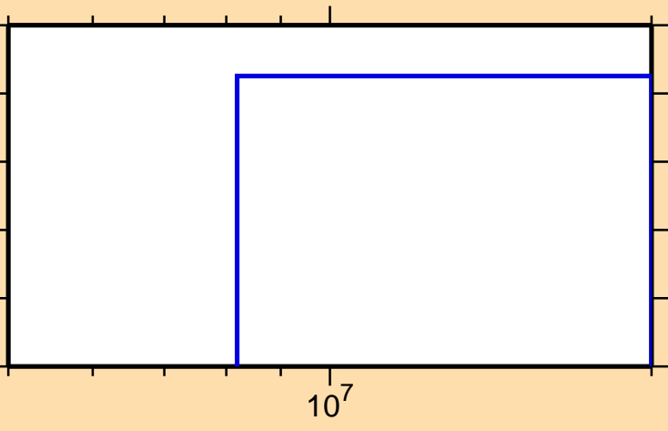
\sigma vs. E for ^{119}\text{Ag}(n,2n\alpha)
