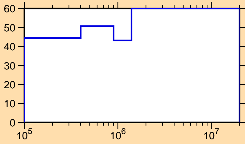
\Delta\sigma/\sigma vs. E for ^{119}\text{Ag}(n,n_1)
