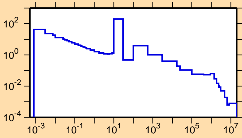
\sigma vs. E for ^{119}\text{Ag}(n,\gamma)
