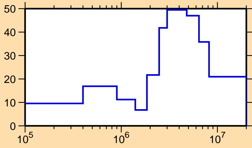
\Delta\sigma/\sigma vs. E for ^{119}\text{Ag}(n,\text{tot.})
