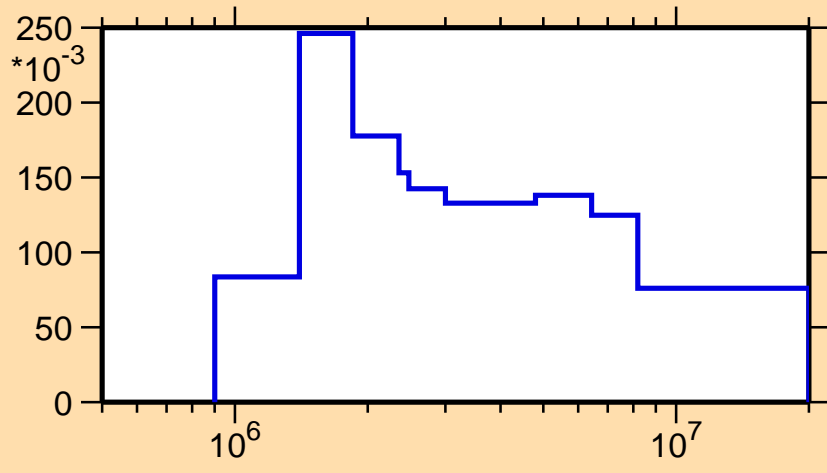
\sigma vs. E for ^{119}\text{Ag}(n,n_2)
