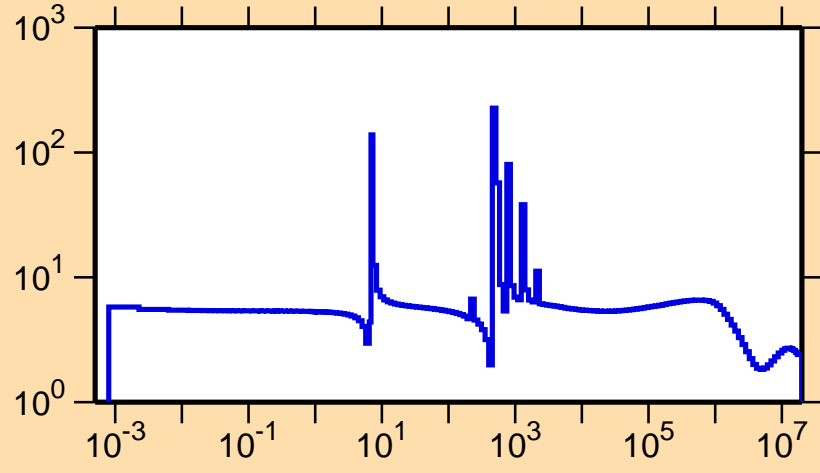
\sigma vs. E for ^{119}\text{Ag}(n,\text{el.})
