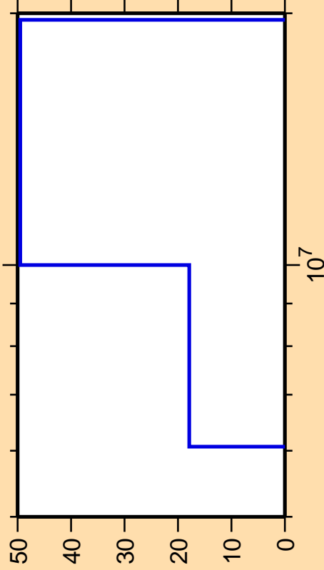
\Delta\sigma/\sigma vs. E for ^{119}\text{Ag}(n,2n)
