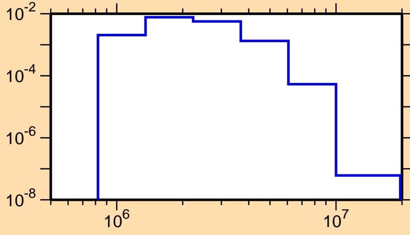
\sigma vs. E for ^{119}\text{Ag}(n,n_3)
