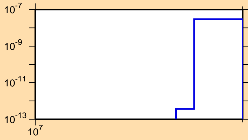
\sigma vs. E for ^{120}\text{Ag}(n,2np)
