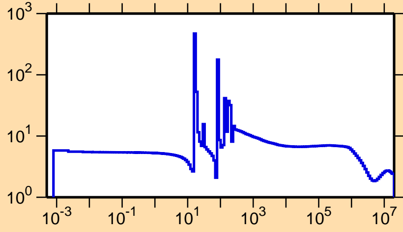
\sigma vs. E for ^{120}\text{Ag}(n,\text{el.})
