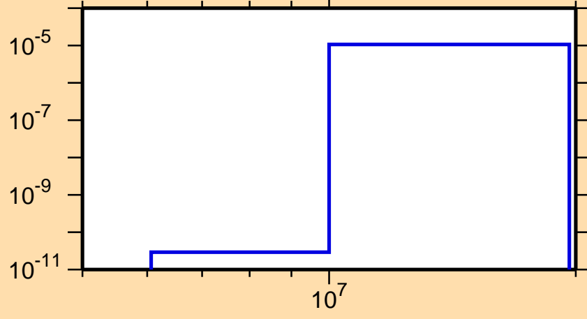
\sigma vs. E for ^{120}\text{Ag}(n,\alpha)
