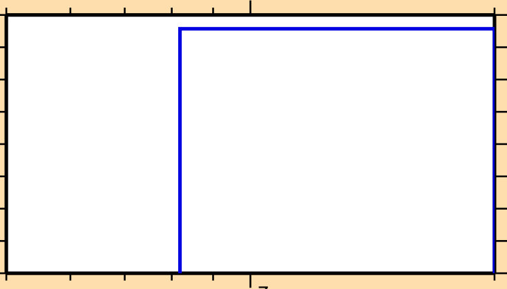
\sigma vs. E for ^{120}\text{Ag}(n,d)
