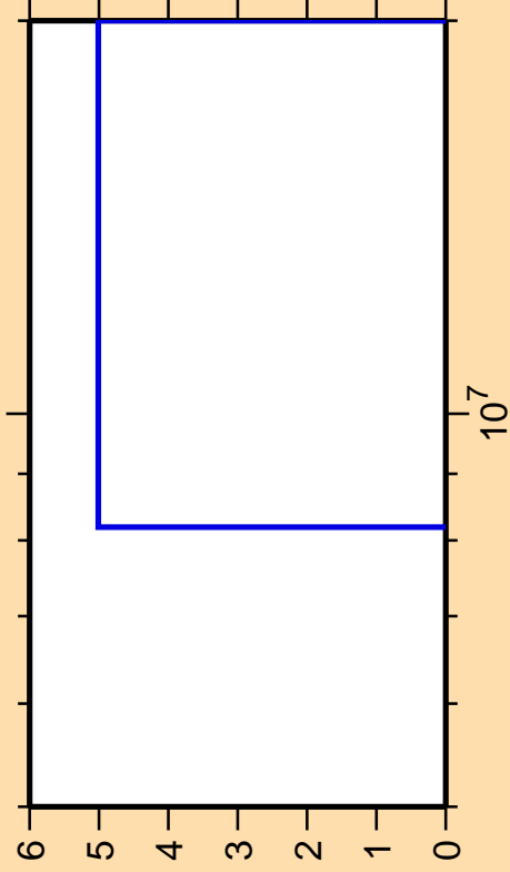
\Delta\sigma/\sigma vs. E for ^{120}\text{Ag}(n,2n\alpha)
