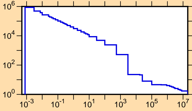
\sigma vs. E for ^{24}\text{Al}(n,\text{tot.})
