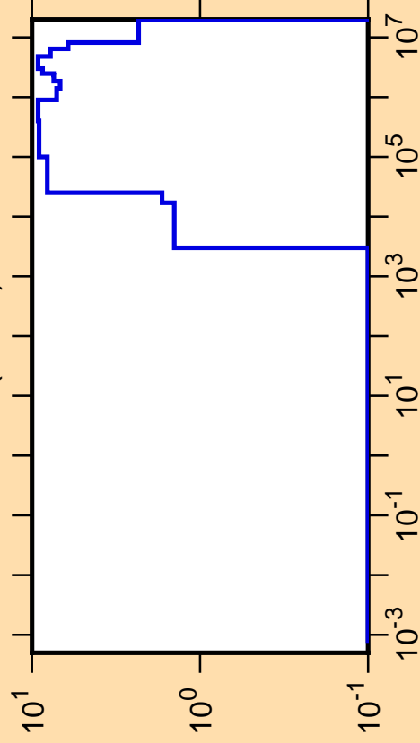
\Delta\sigma/\sigma vs. E for ^{24}\text{Al}(n,\text{tot.})
