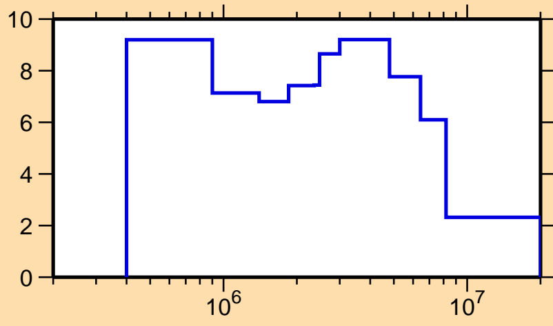
\Delta\sigma/\sigma vs. E for ^{24}\text{Al}(n,\text{tot.})
