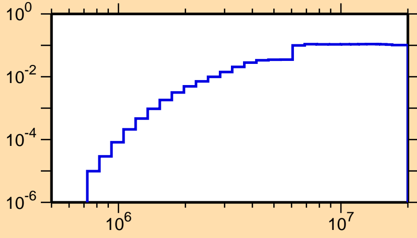
\sigma vs. E for ^{25}\text{Al}(n,d)
