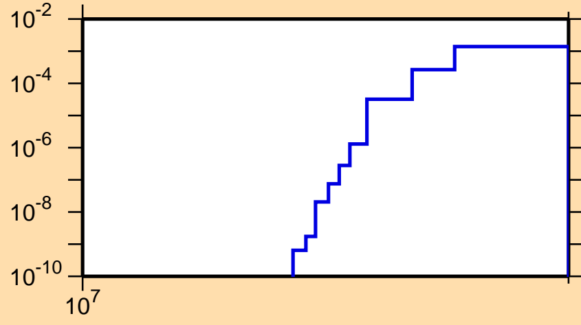
\sigma vs. E for ^{25}\text{Al} (mt 45)
