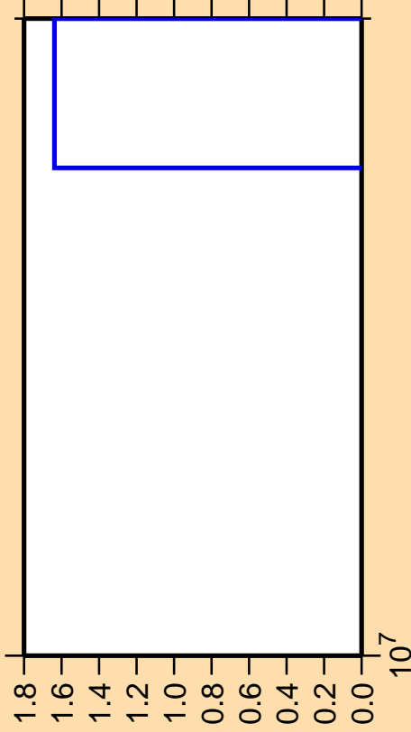
\Delta\sigma/\sigma vs. E for ^{25}\text{Al}(n,2np)
