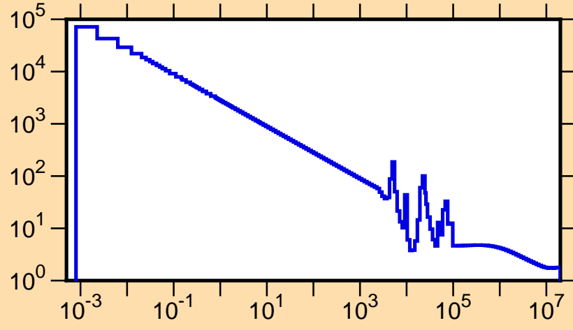
\sigma vs. E for ^{25}\text{Al}(n,\text{tot.})
