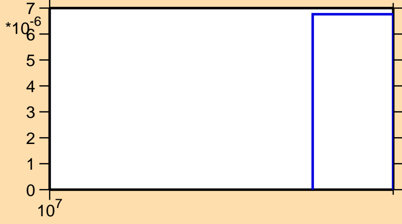
\sigma vs. E for ^{25}\text{Al}(n,2n)
