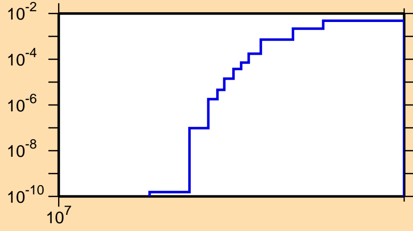
\sigma vs. E for ^{25}\text{Al}(n,\text{pd})
