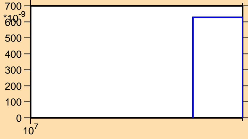
\sigma vs. E for ^{25}\text{Al}(n,nd)
