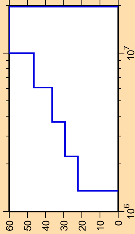
\Delta\sigma/\sigma vs. E for ^{25}\text{Al}(n,n_4)
