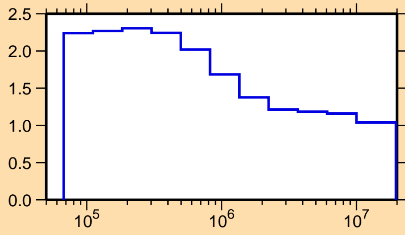
\sigma vs. E for ^{25}\text{Al}(n,\text{nonel.})
