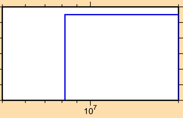
\sigma vs. E for ^{25}\text{Al}(n,2n)
