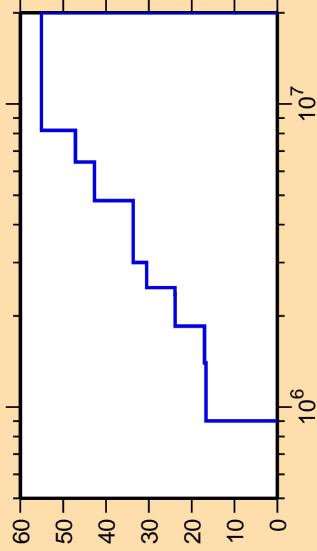
\Delta\sigma/\sigma vs. E for ^{25}\text{Al}(n,n_2)
