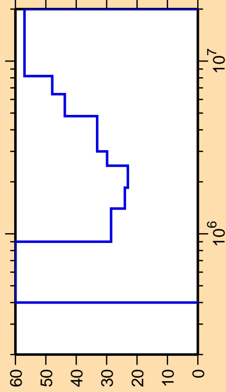
\Delta\sigma/\sigma vs. E for ^{25}\text{Al}(n,\text{inel.})
