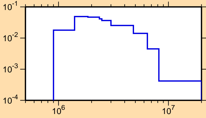
\sigma vs. E for ^{25}\text{Al}(n,n_2)
