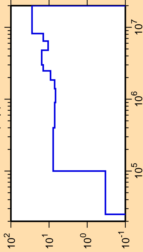
\Delta\sigma/\sigma vs. E for ^{25}\text{Al}(n,p)
