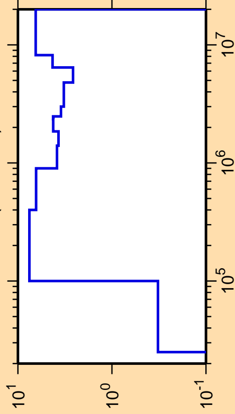
\Delta\sigma/\sigma vs. E for ^{25}\text{Al}(n,\text{nonel.})
