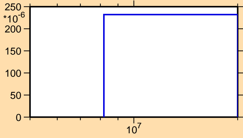
\sigma vs. E for ^{25}\text{Al}(n,\text{pd})
