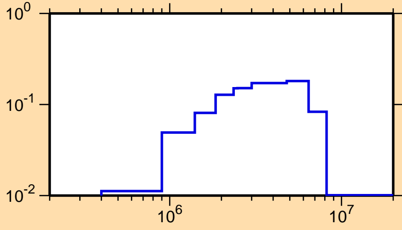
\sigma vs. E for ^{25}\text{Al}(n,\text{inel.})
