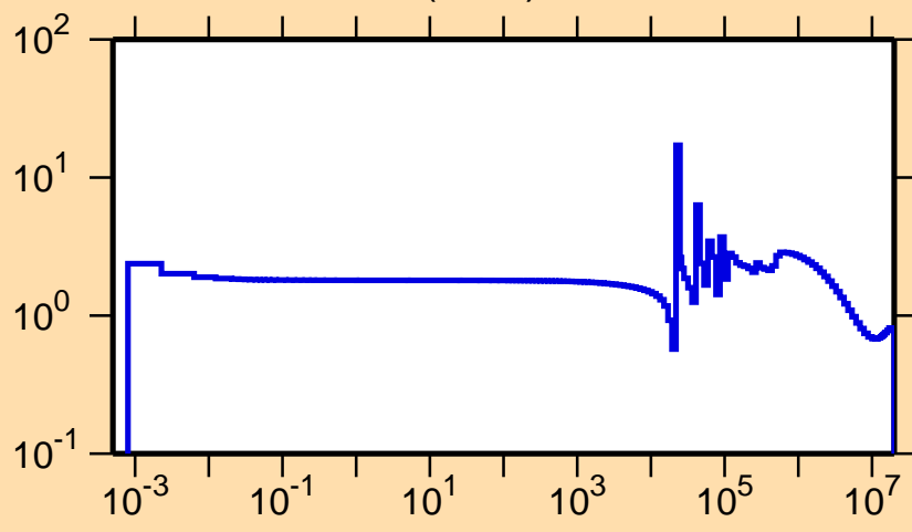
\sigma vs. E for ^{26}\text{Al}(n,\text{el.})
