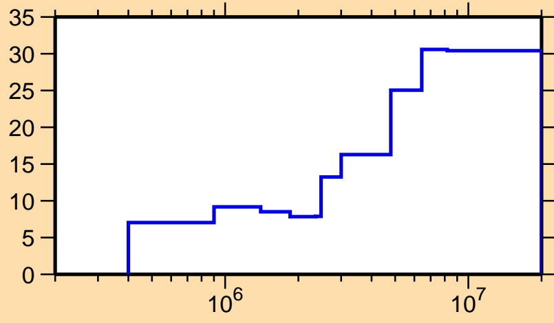
\Delta\sigma/\sigma vs. E for ^{26}\text{Al}(n,p)
