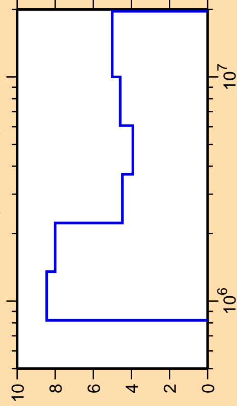
\Delta\sigma/\sigma vs. E for ^{27}\text{Al}(n,\text{nonel.})
