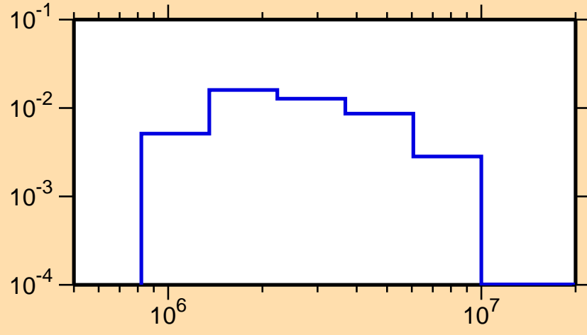
\sigma vs. E for ^{28}\text{Al}(n,n_2)
