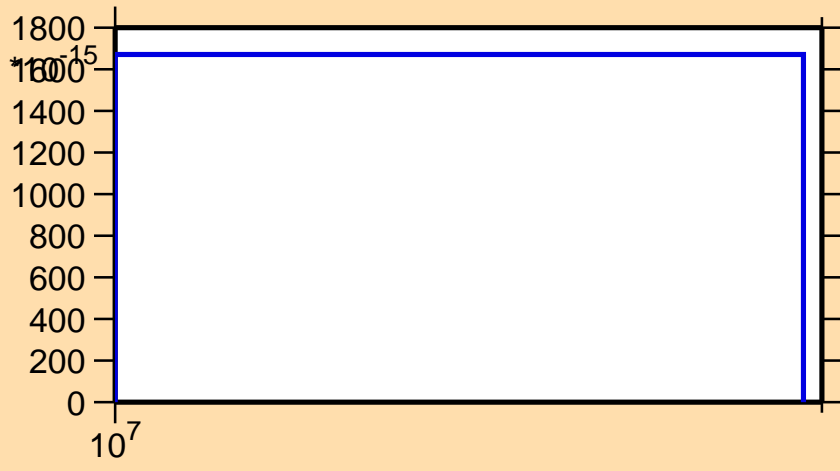
\sigma vs. E for ^{28}\text{Al}(n,2n\alpha)
