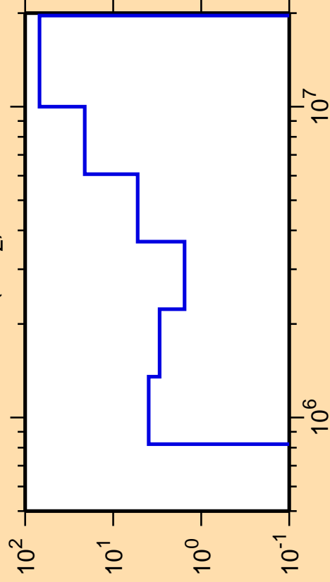
\Delta\sigma/\sigma vs. E for ^{28}\text{Al}(n,n_2)
