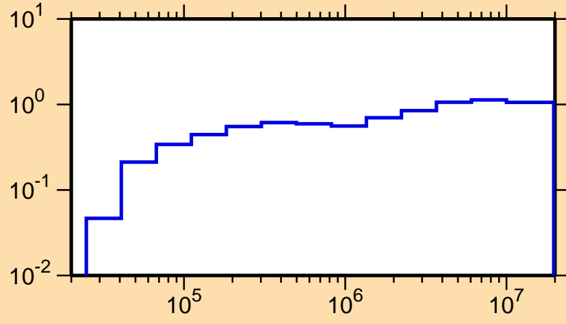
\sigma vs. E for ^{28}\text{Al}(n,\text{nonel.})
