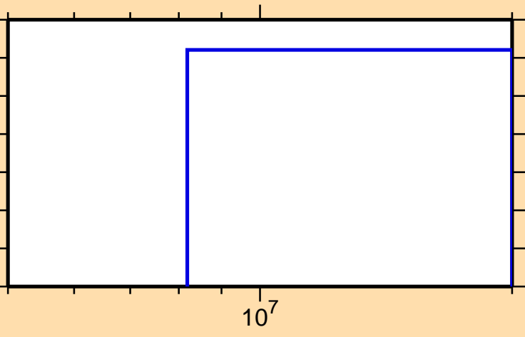
\sigma vs. E for ^{28}\text{Al}(n,p\alpha)
