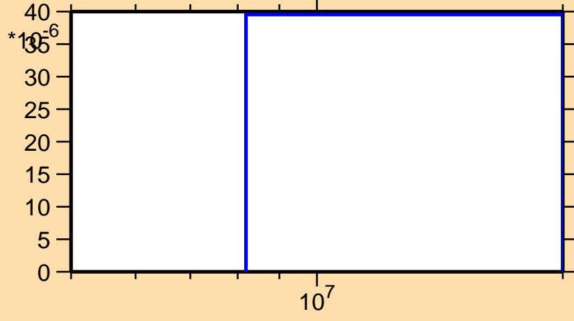
\sigma vs. E for ^{28}\text{Al}(n,nd)
