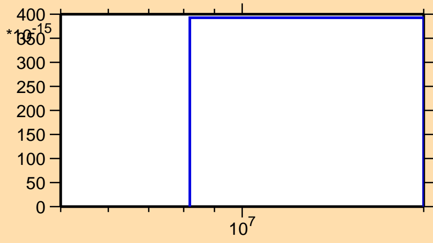
\sigma vs. E for ^{28}\text{Al}(n,nt)
