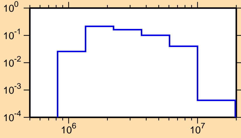
\sigma vs. E for ^{30}\text{Al}(n,n_4)
