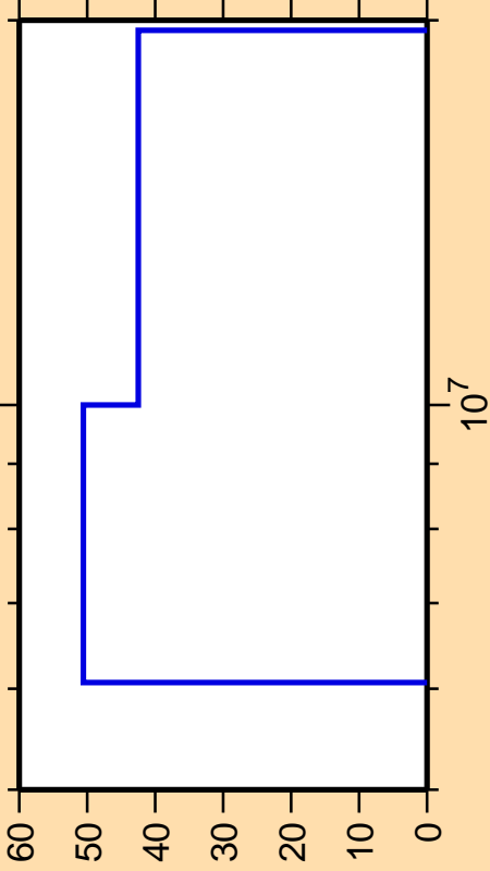
\Delta\sigma/\sigma vs. E for ^{30}\text{Al}(n,p)
