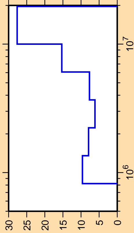
\Delta\sigma/\sigma vs. E for ^{30}\text{Al}(n,n_4)
